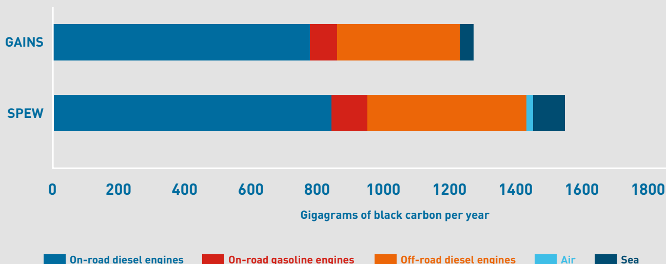
Figure 4 Estimated global black carbon emissions from transportation from the SPEW and GAINS models in Bond’s 2013 study. Note that the category of “off-road diesel engines” includes rail and sea transport, as well as other heavy machinery and agricultural vehicles.
